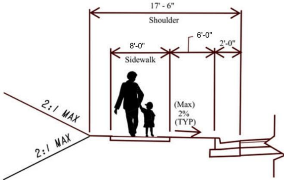
TYPICAL SECTION
