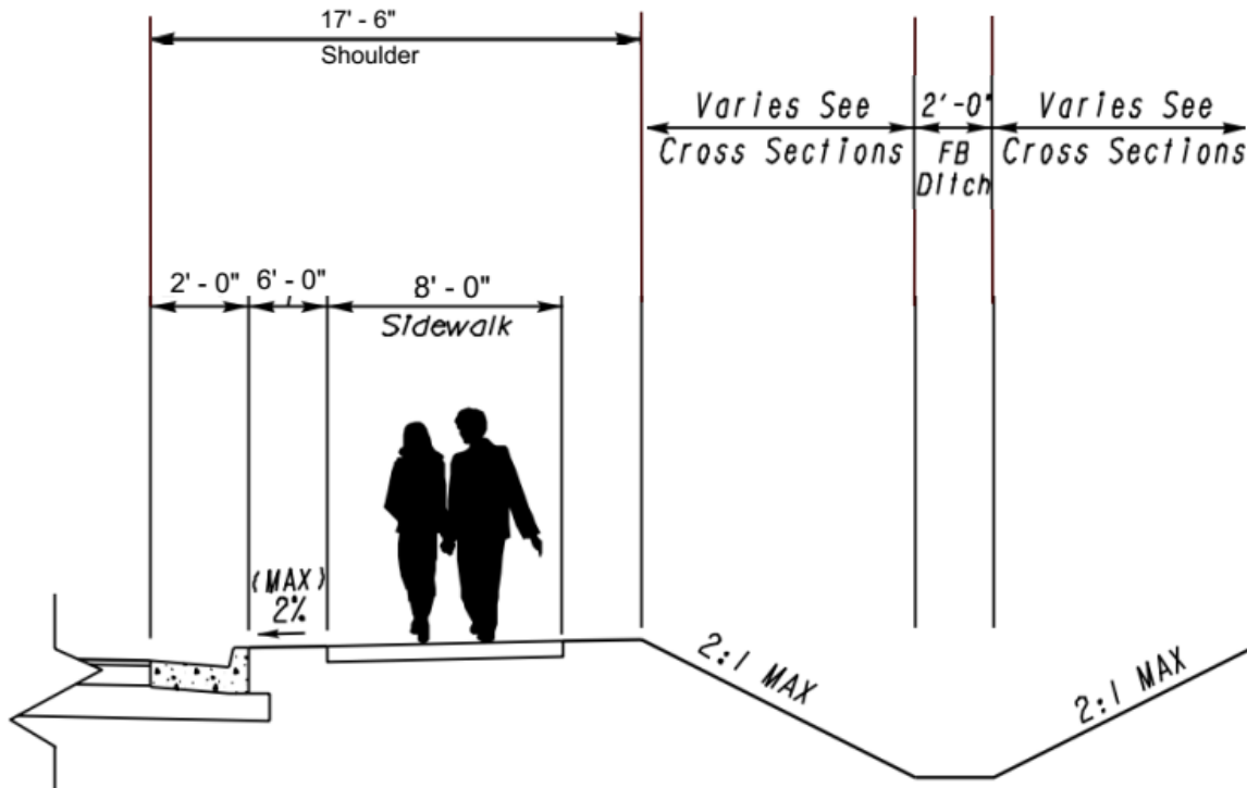
TYPICAL SECTION APPLIES TO PROPOSED DAVIS DRIVE ALTERNATE #2
